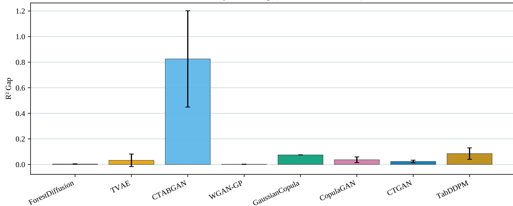
Air Quality — R^2 Gap (mean \pm SD, 10 seeds)
